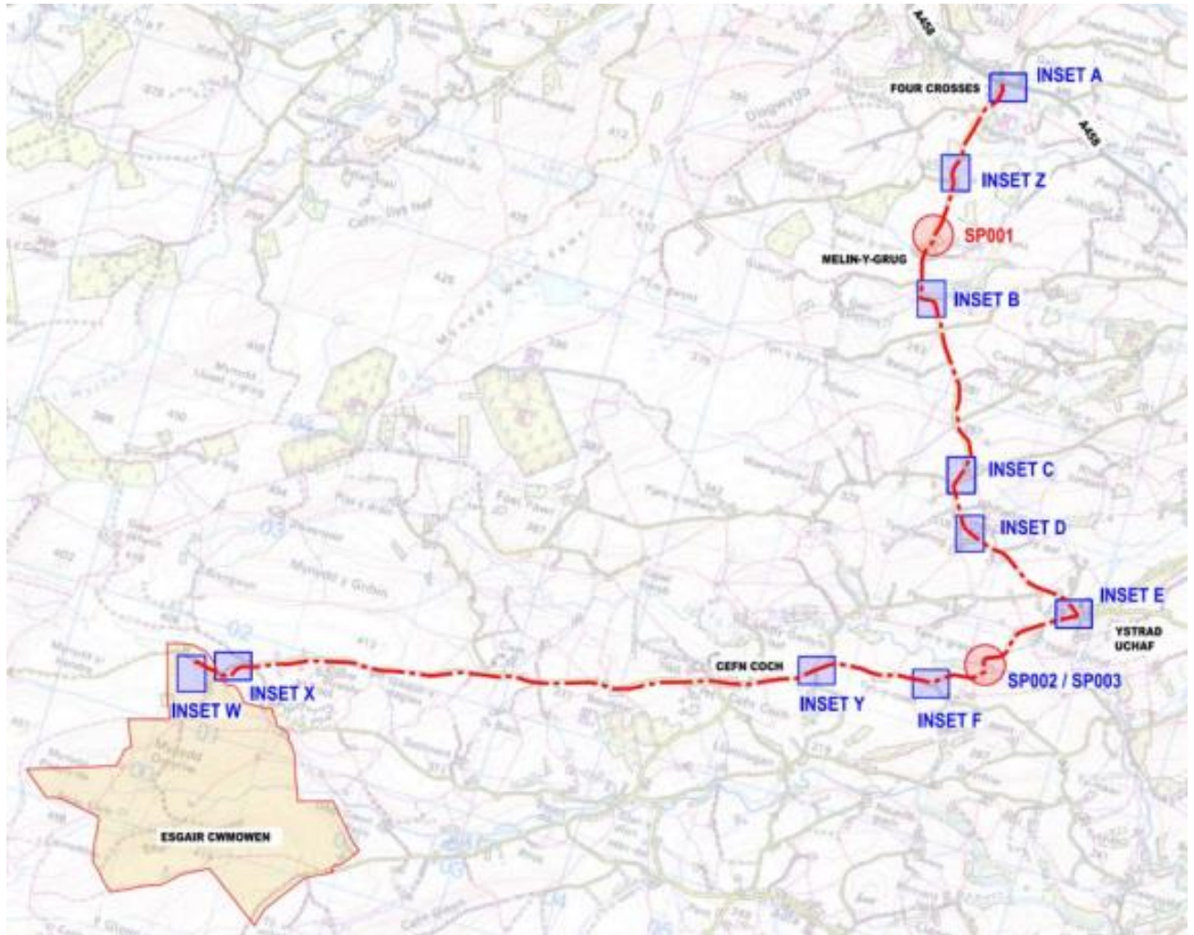
TRAFFIC PLAN (route for lorry traffic – large elements may use A470)
